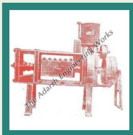
Small Scale Oil Expellers
