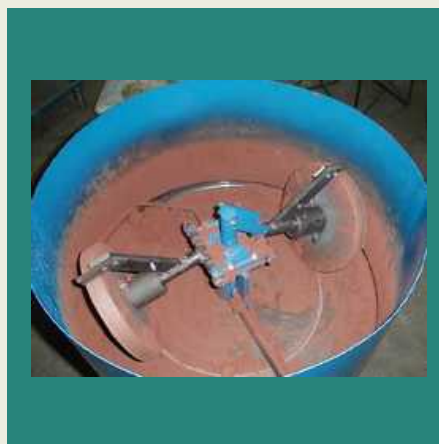
Sand Muller Mixer for Foundry Industries
